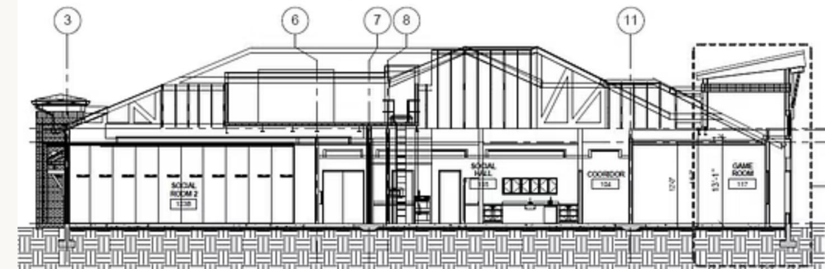
(C) OVERALL BUILDING SECTION SCALE: 1/8" = 1'-0"
