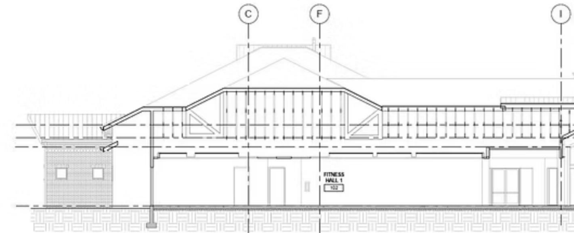
(A) OVERALL BUILDING SECTION SCALE: 1/8" = 1'-0"
