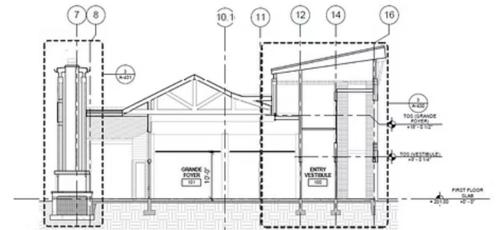
(B) OVERALL BUILDING SECTION SCALE: 1/8" = 1'-0"
